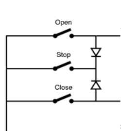
2 Normally Open contact + Stop in parallel
